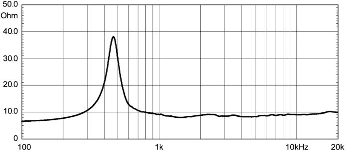
ND1424BT MEASURED WITH 1W INPUT ON RATED IMPEDANCE AT 1 M DISTANCE ON AXIS FROM THE MOUTH OF XT1464 HORN FREE AIR IMPEDANCE MAGNITUDE CURVE
